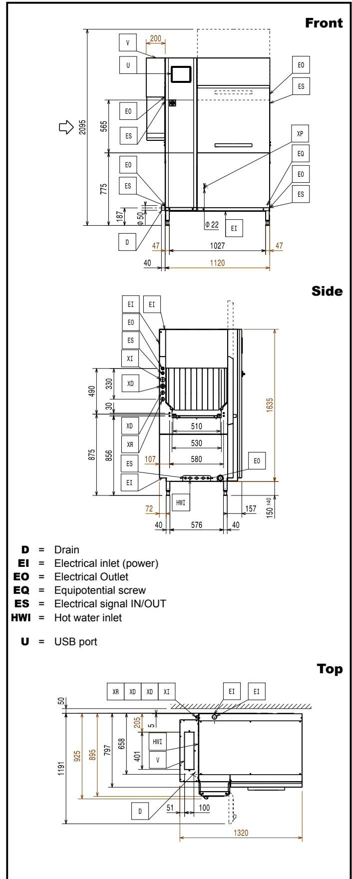
Warewashing Dual rinse rack type dishwasher, 150 racks/hour, electric, 50Hz
